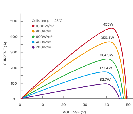
Power-Voltage Curve
